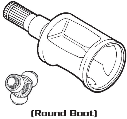
Tripod Type (Round Housing)
